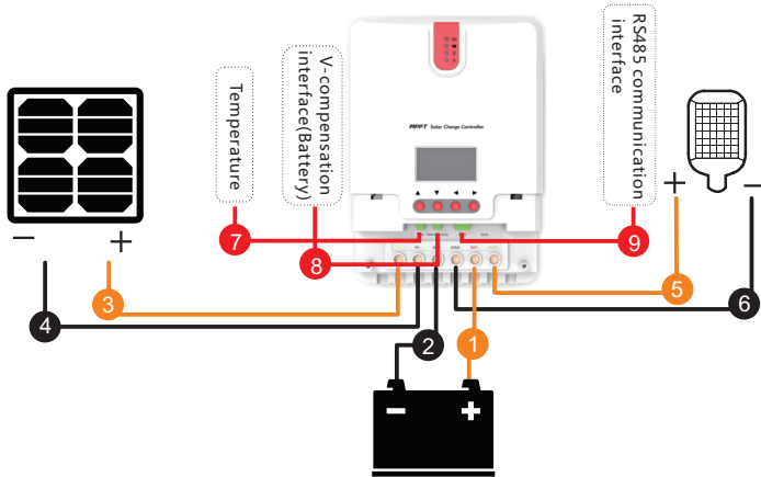
Fig. 2.3 Wiring sequence
